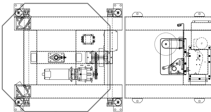
Typical Predator SS HP with scale
