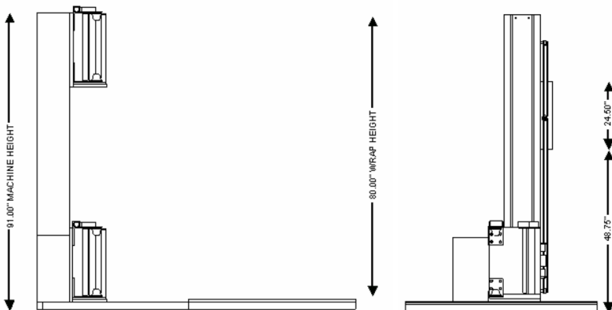
Figure 1A: Predator SS Low Profile Scale Overview Layout
