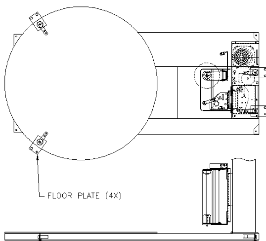
Typical Predator SS with scale
