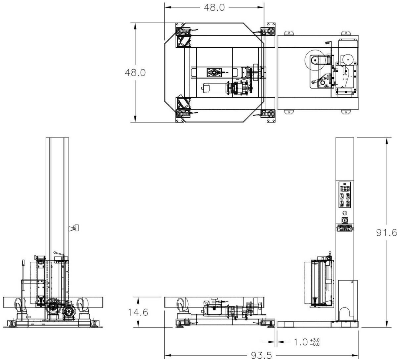
Figure 1B: Predator SS High Profile Scale Overview Layout
