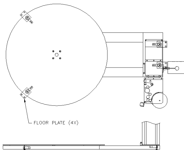
Typical Predator XS with scale
